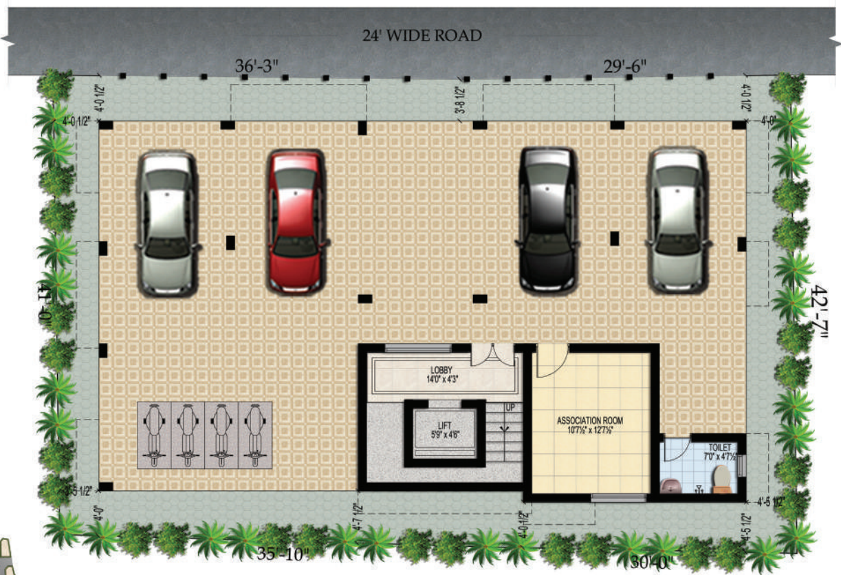
BLOCK - B (1&2) STILT FLOOR PLAN
